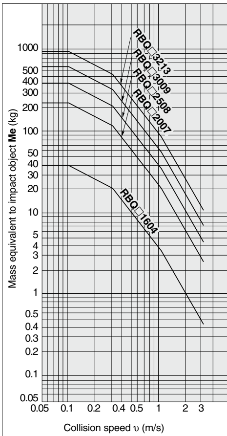
Corresponding Mass of Impacting Object M_e
