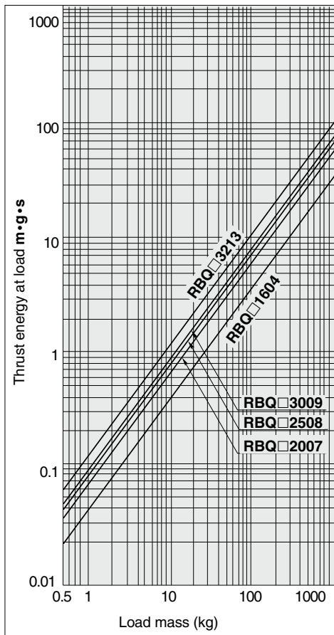
Thrust Energy at Load m \cdot g \cdot s
